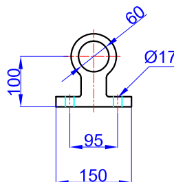
47000057-0001 (Bracket Kits T 60-100-150-22)
