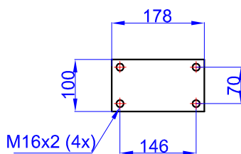
47000028-02-001 (Bracket Kits Top Clevis GHTC GEZ 50x80)
