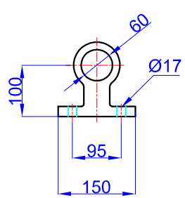
4700057-0001 (Bracket Kits T 60-100-150-22)
